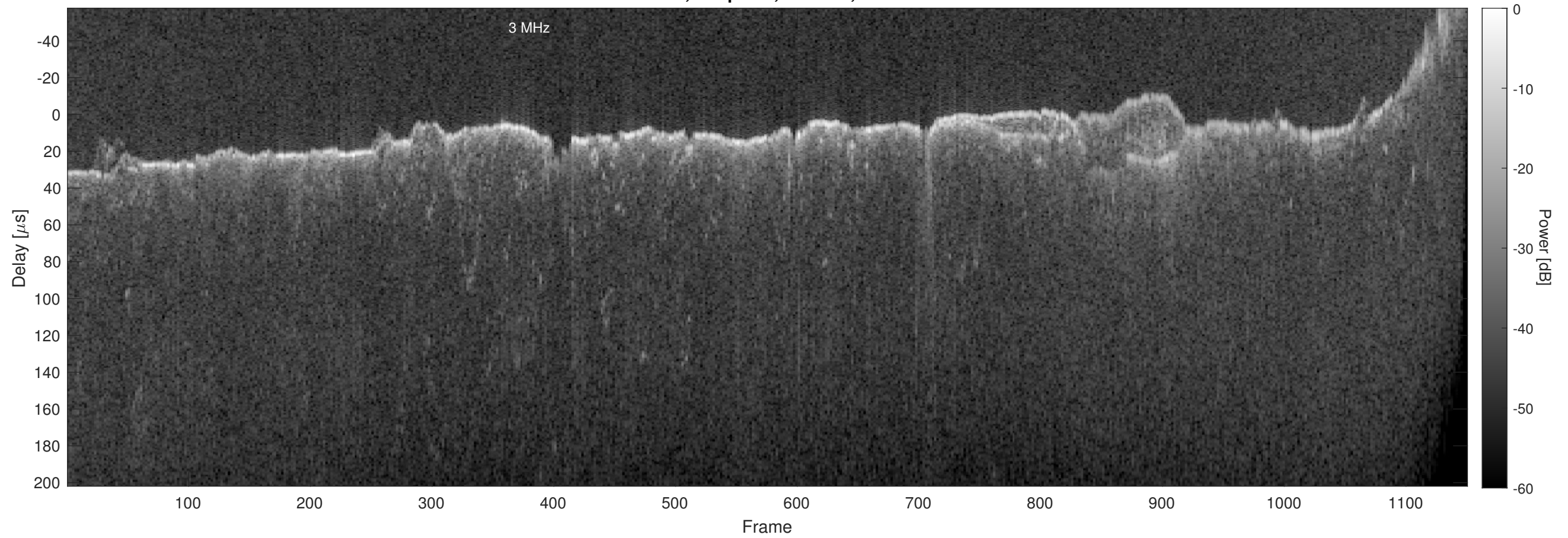
Orbit 15166, Chapman, Window, Channel 2
