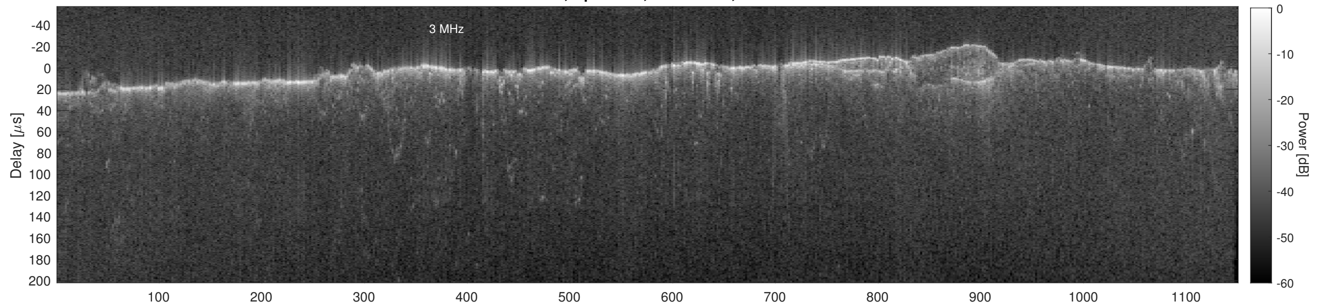
Orbit 15166, Cluttergram
