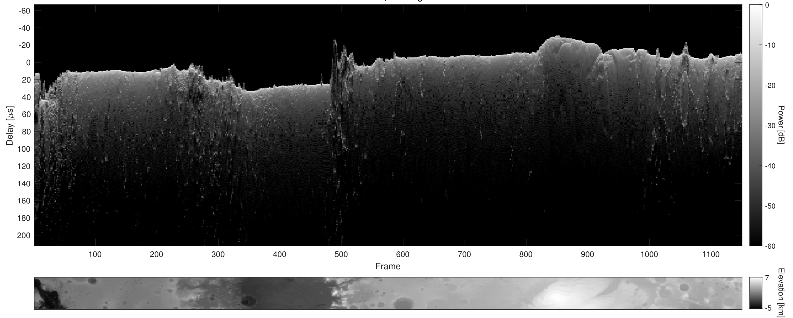
Orbit 15172, Cluttergram
