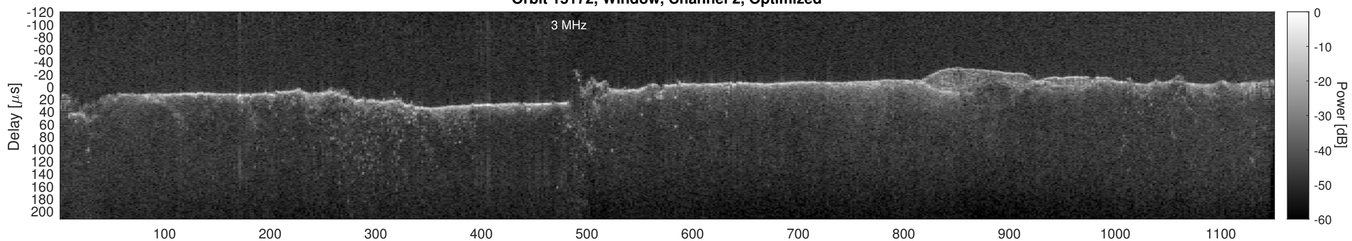
Orbit 15172, Cluttergram
