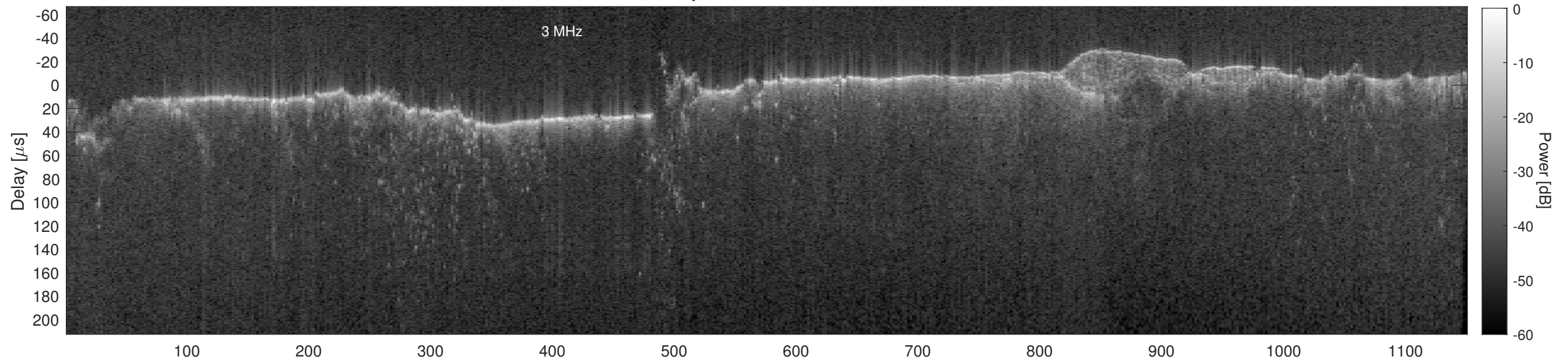
Orbit 15172, Cluttergram
