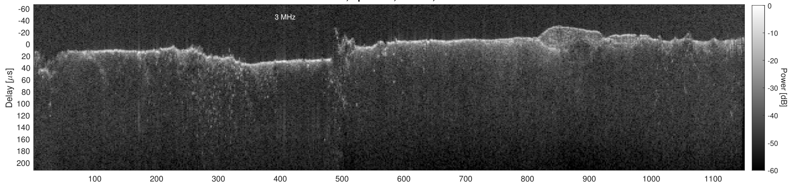
Orbit 15172, Cluttergram
