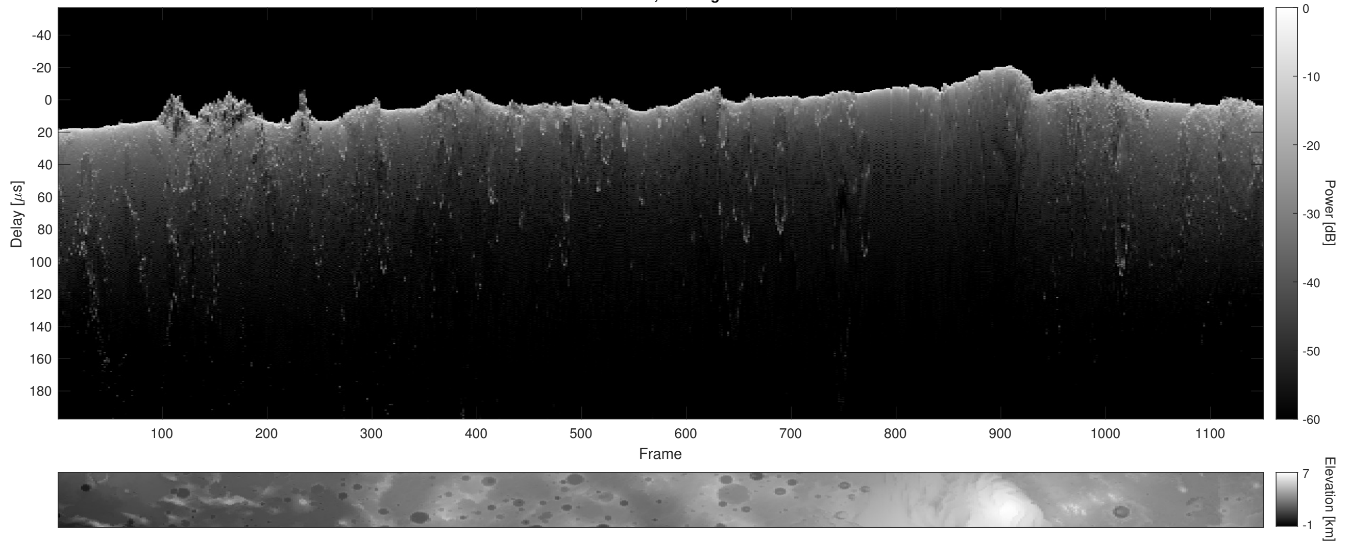
Orbit 15173, Cluttergram
