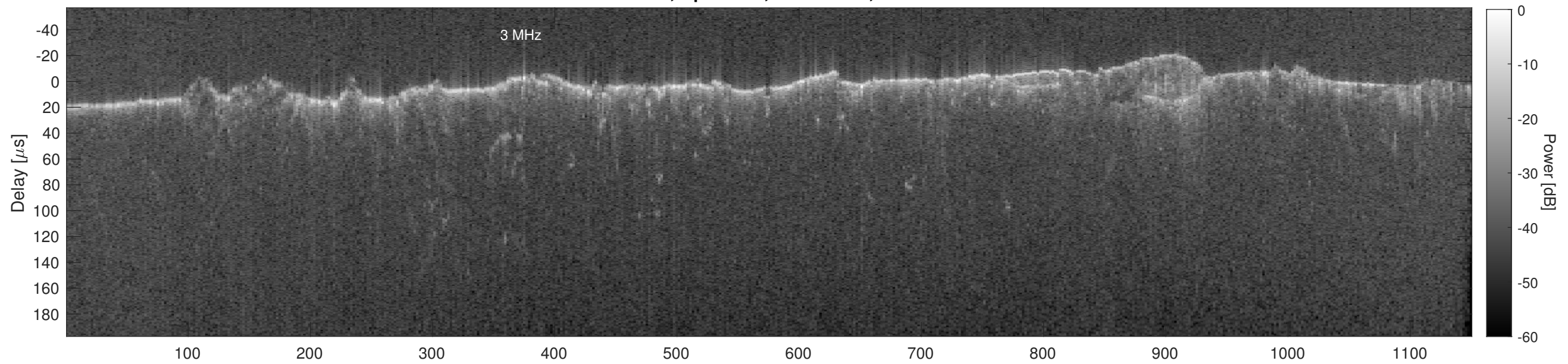
Orbit 15173, Cluttergram
