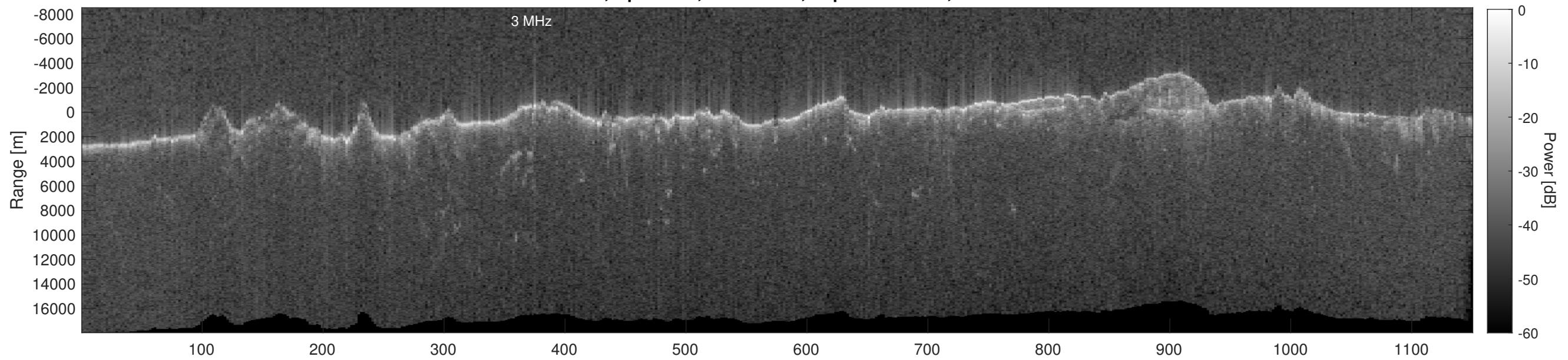
Orbit 15173, Depth-Corrected Cluttergram
