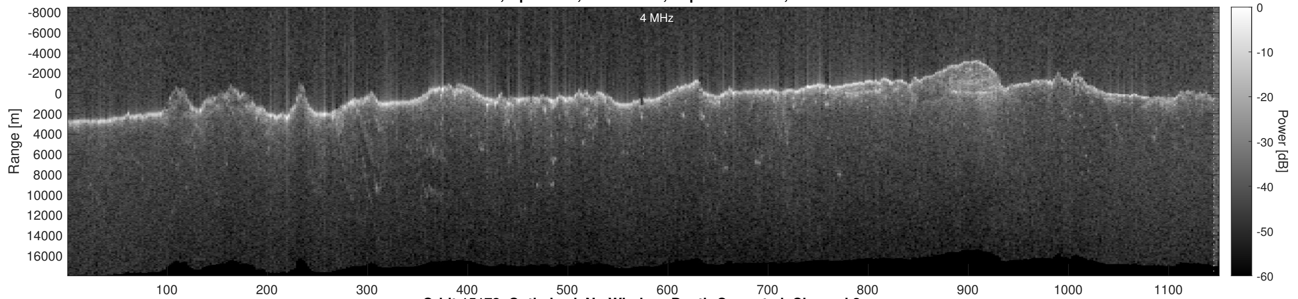
Orbit 15173, Optimized, No Window, Depth-Corrected, Channel 2
