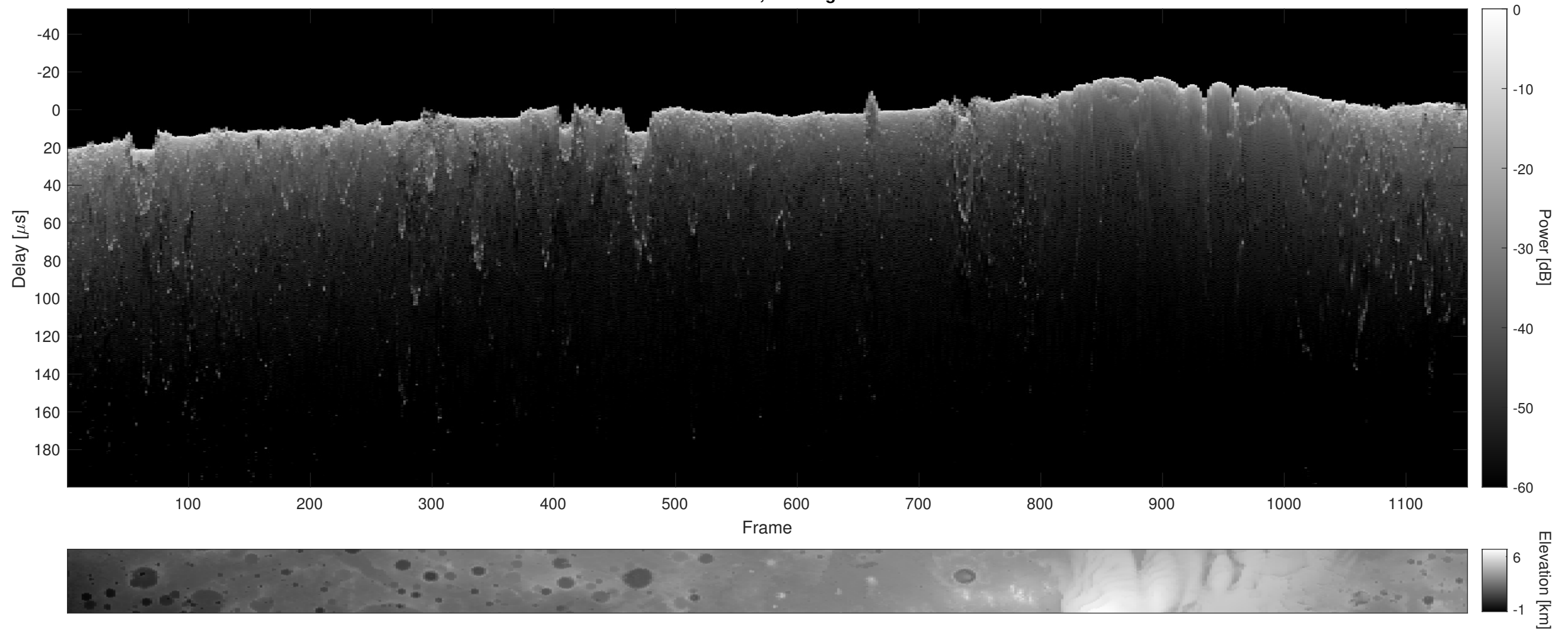
Orbit 15175, Cluttergram
