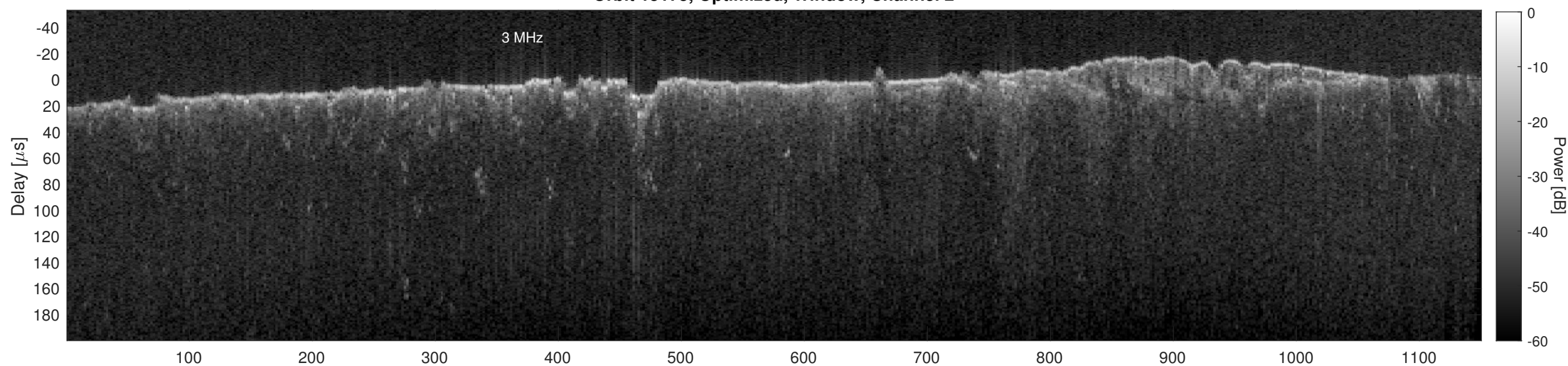
Orbit 15175, Cluttergram
