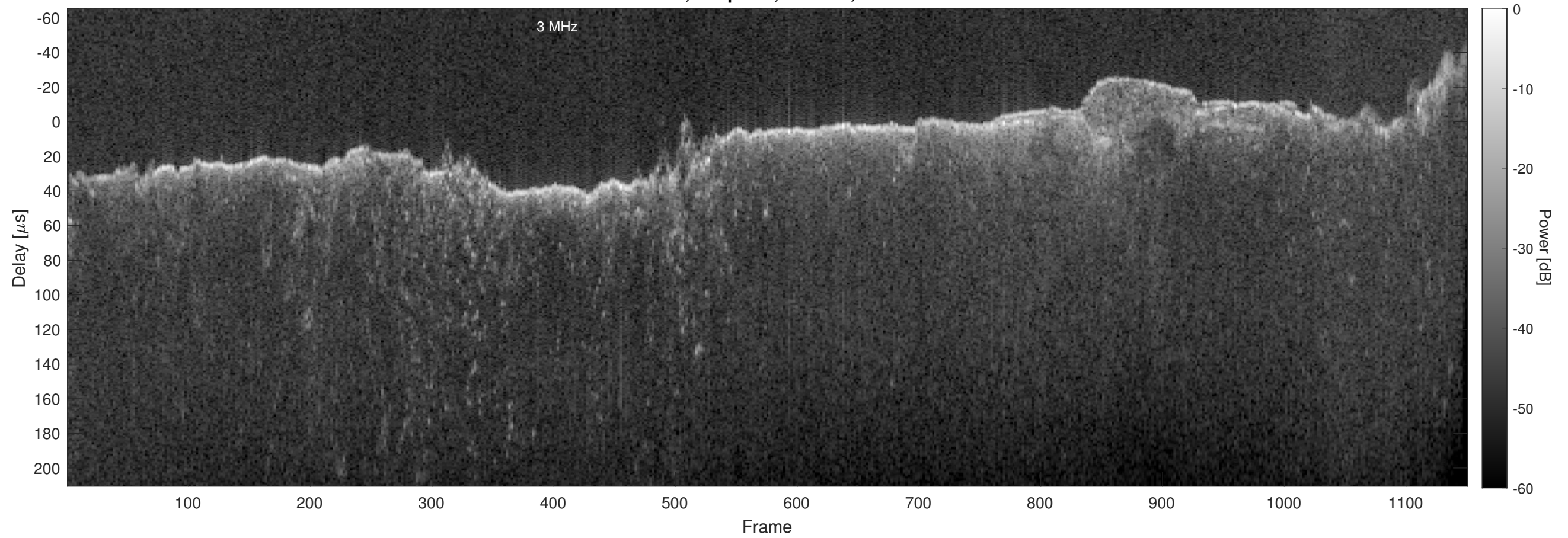
Orbit 15179, Chapman, Window, Channel 2
