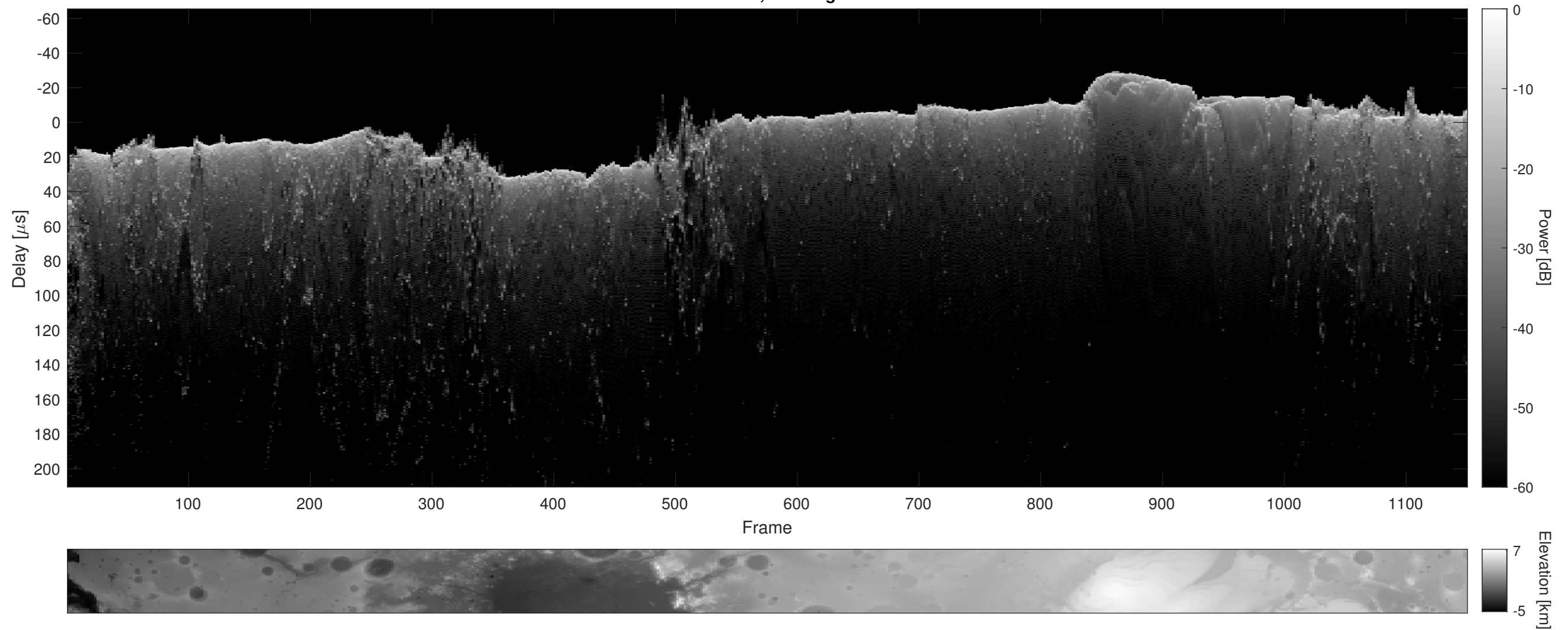
Orbit 15179, Cluttergram
