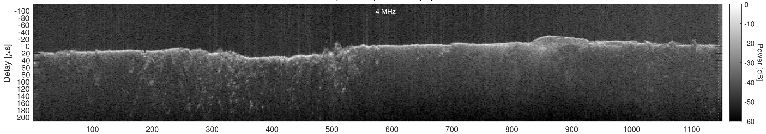
Orbit 15179, Cluttergram
