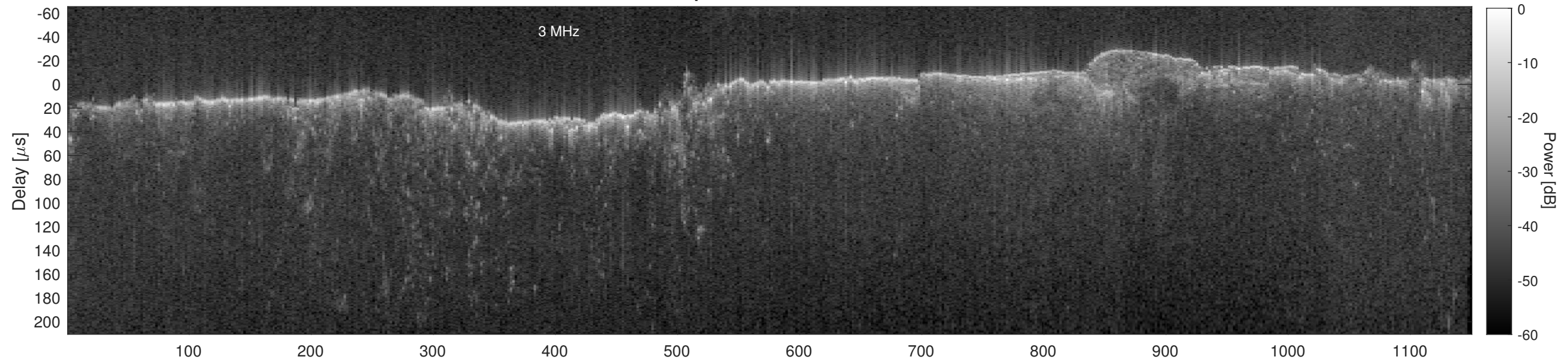
Orbit 15179, Cluttergram
