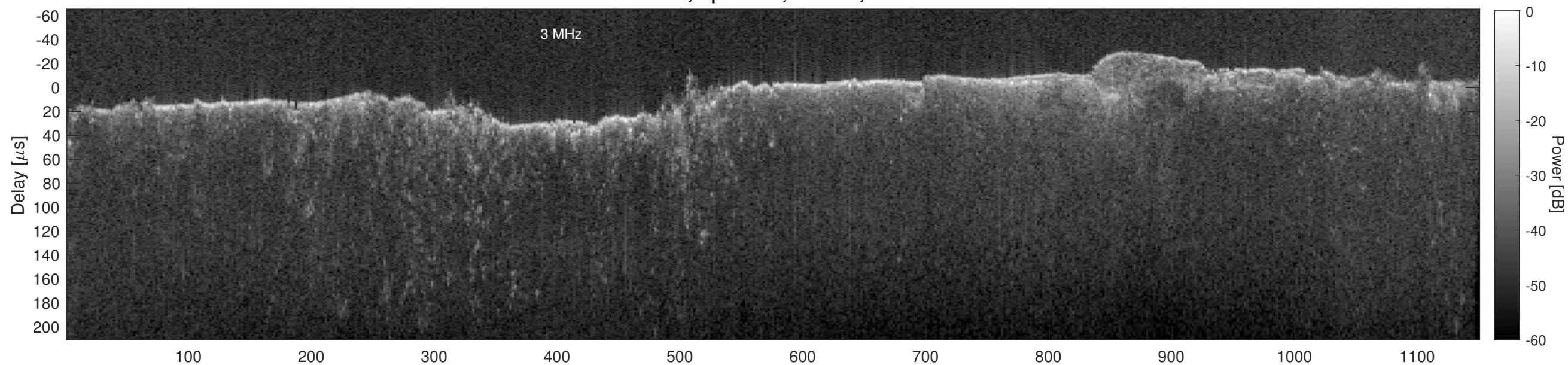
Orbit 15179, Cluttergram
