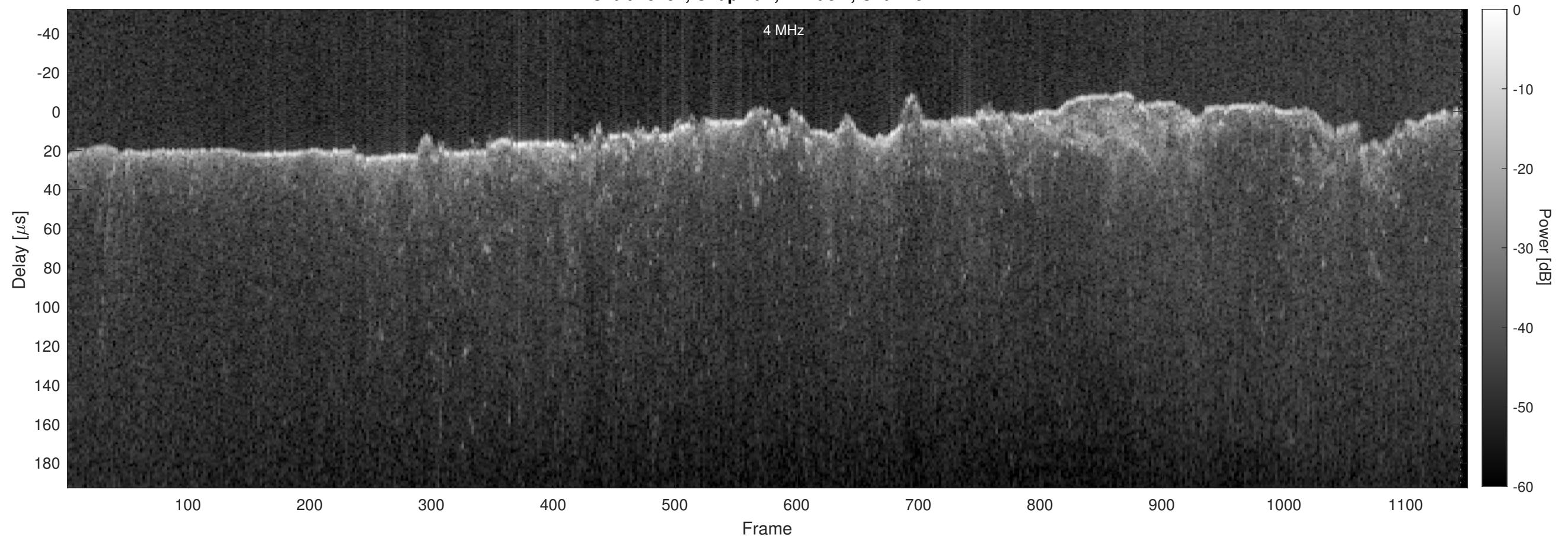
Orbit 15181, Chapman, Window, Channel 2
