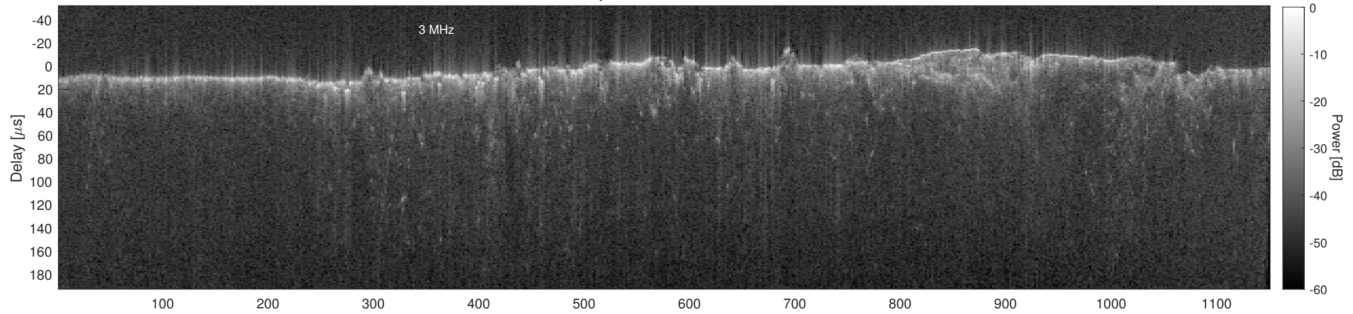
Orbit 15181, Cluttergram
