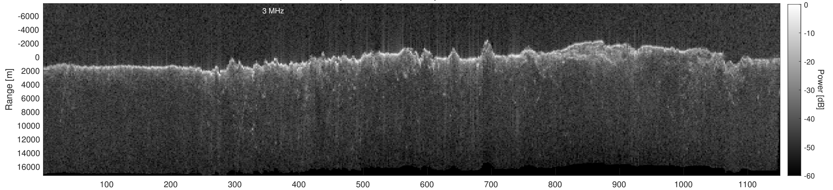
Orbit 15181, Depth-Corrected Cluttergram
