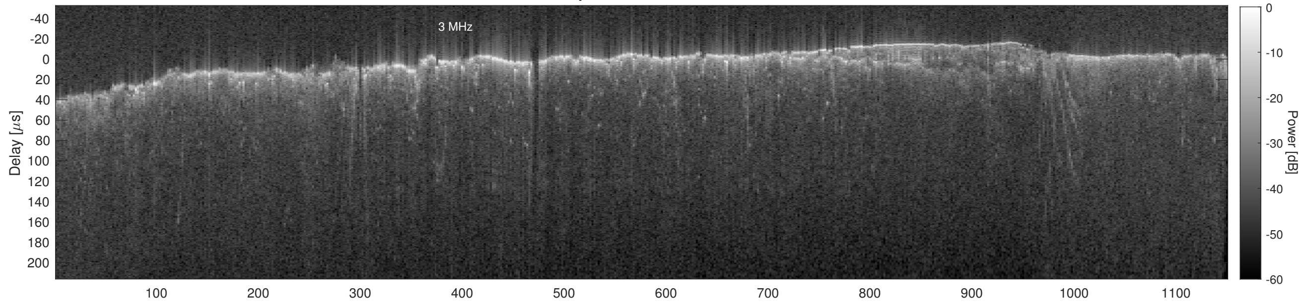
Orbit 15184, Cluttergram
