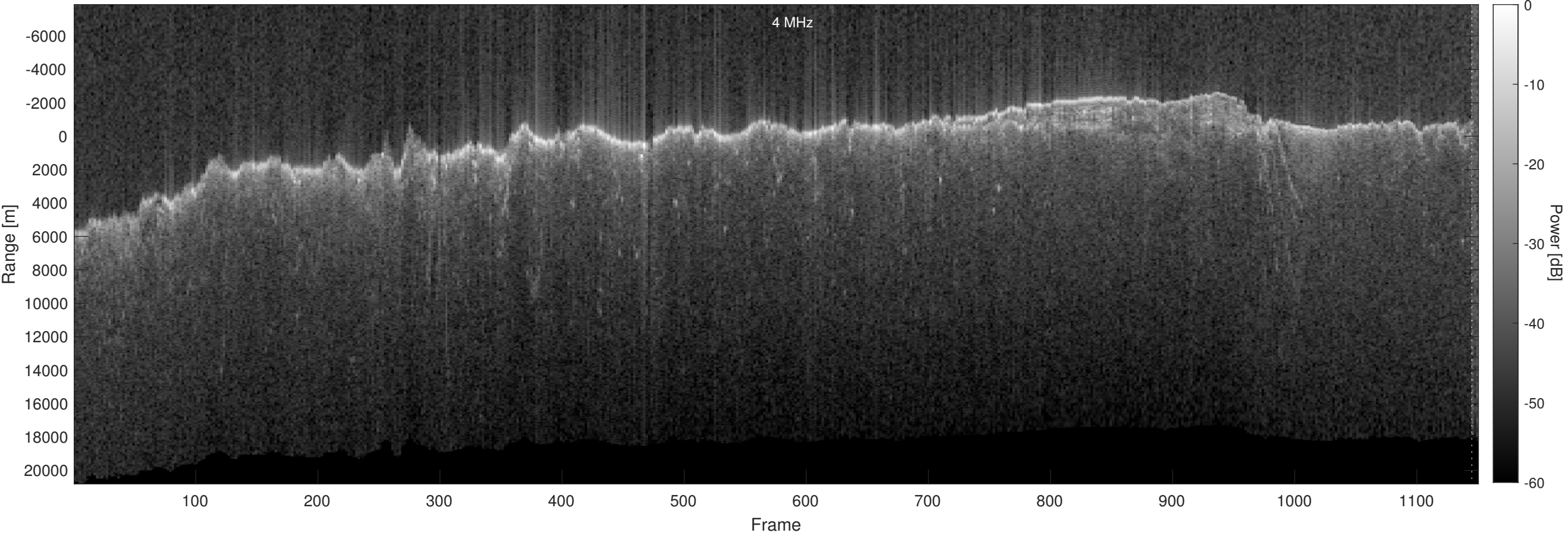
Orbit 15184, Optimized, No Window, Depth-Corrected, Channel 2
