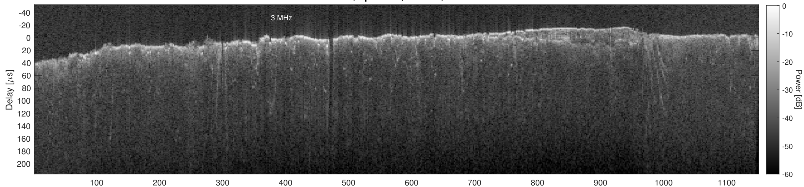
Orbit 15184, Cluttergram
