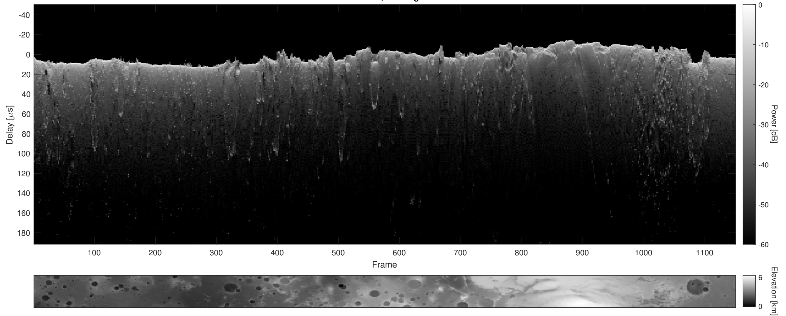
Orbit 15188, Cluttergram
