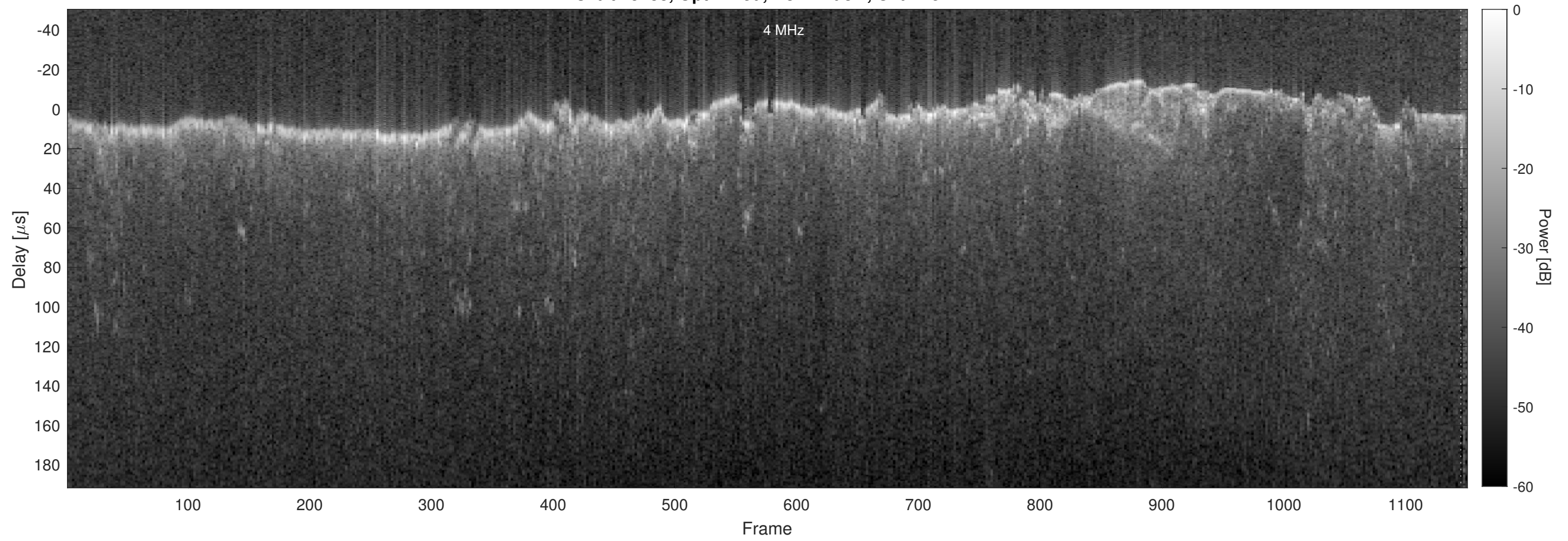
Orbit 15188, Optimized, No Window, Channel 2
