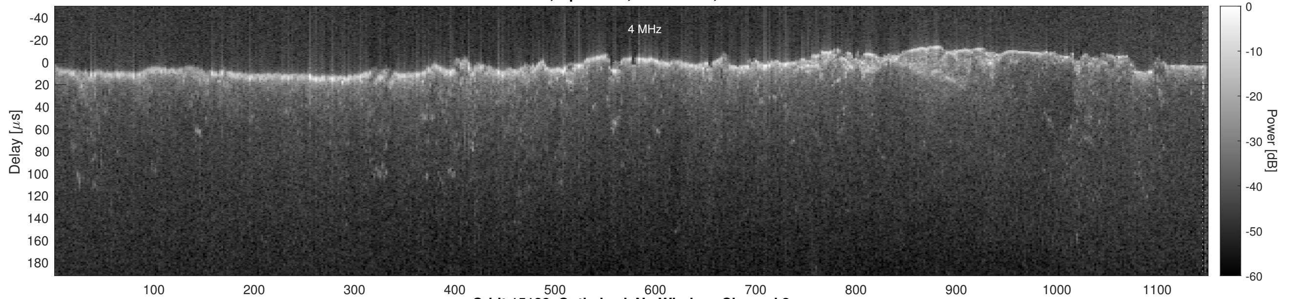
Orbit 15188, Optimized, No Window, Channel 2
