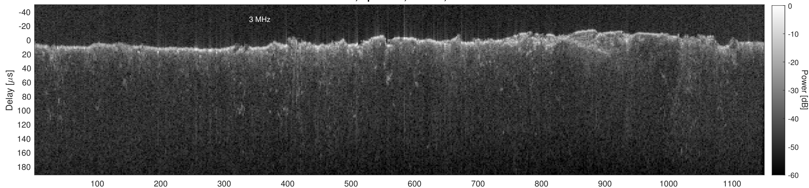
Orbit 15188, Cluttergram
