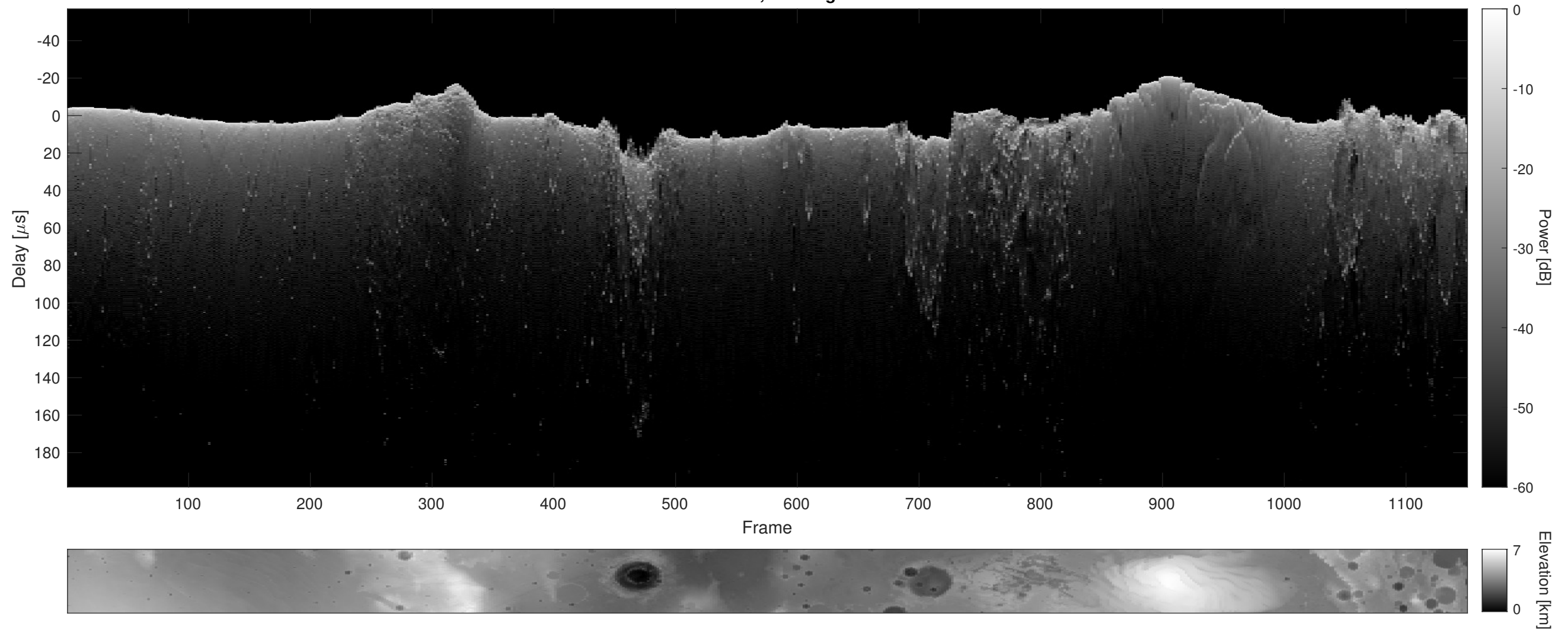
Orbit 15190, Cluttergram
