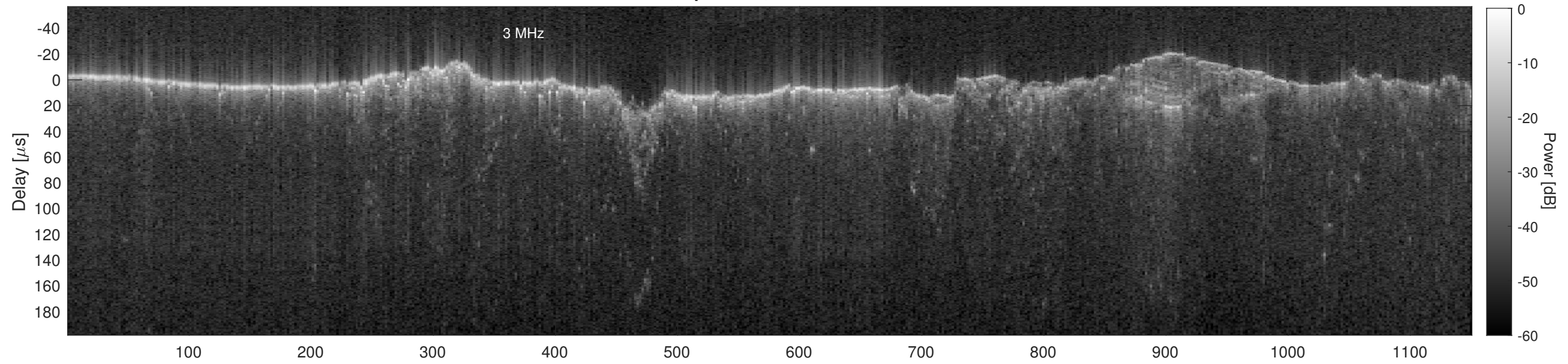
Orbit 15190, Cluttergram
