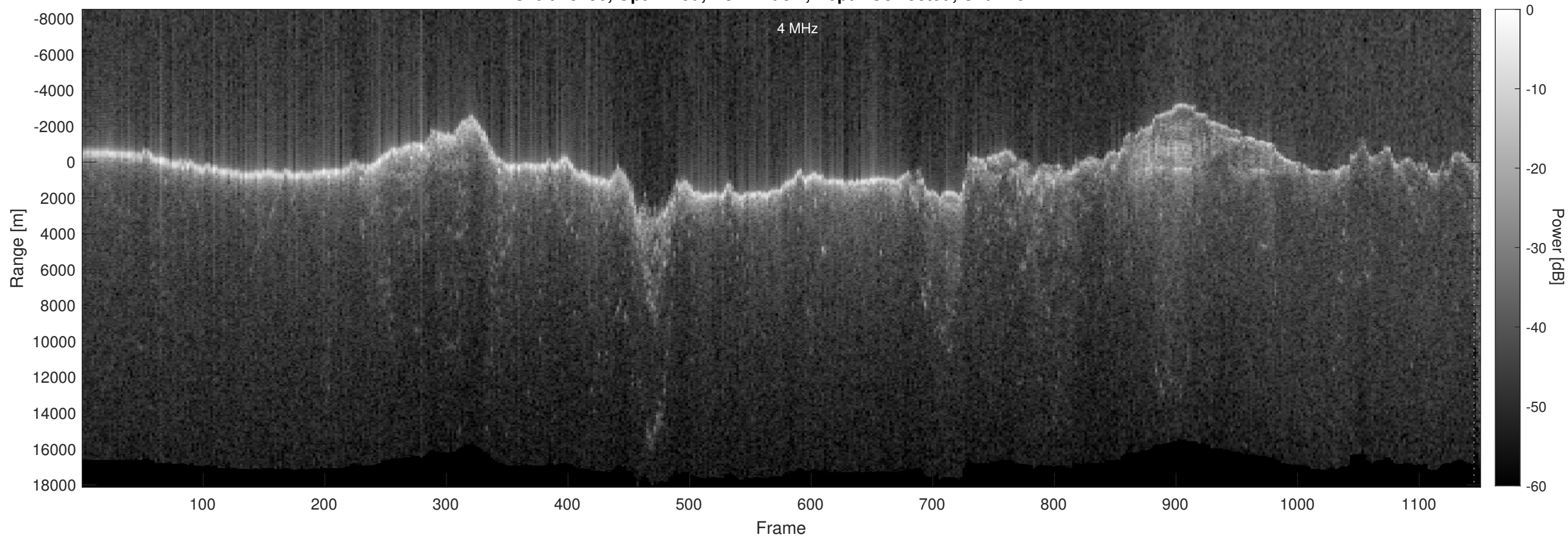
Orbit 15190, Optimized, No Window, Depth-Corrected, Channel 2
