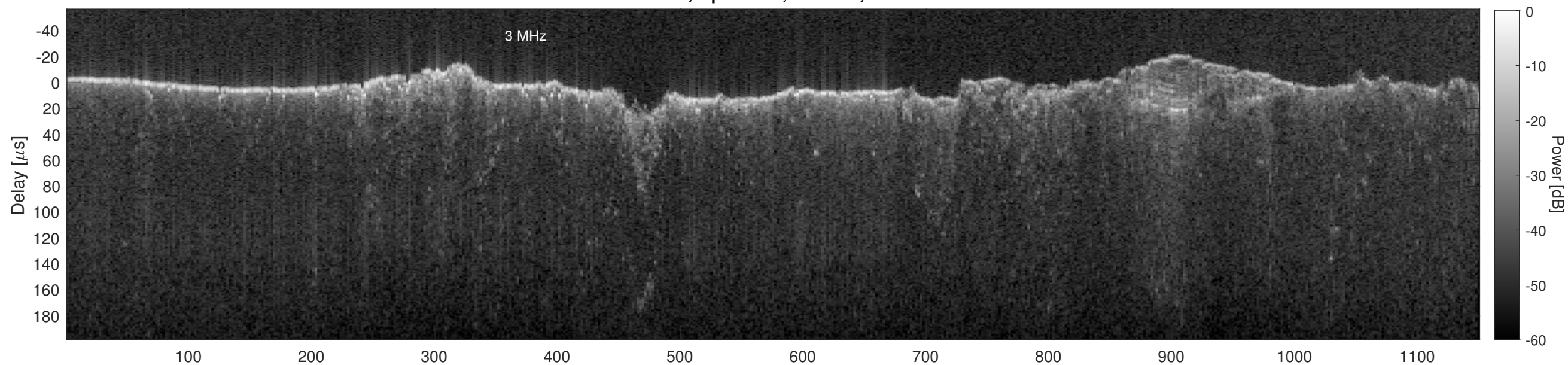
Orbit 15190, Cluttergram
