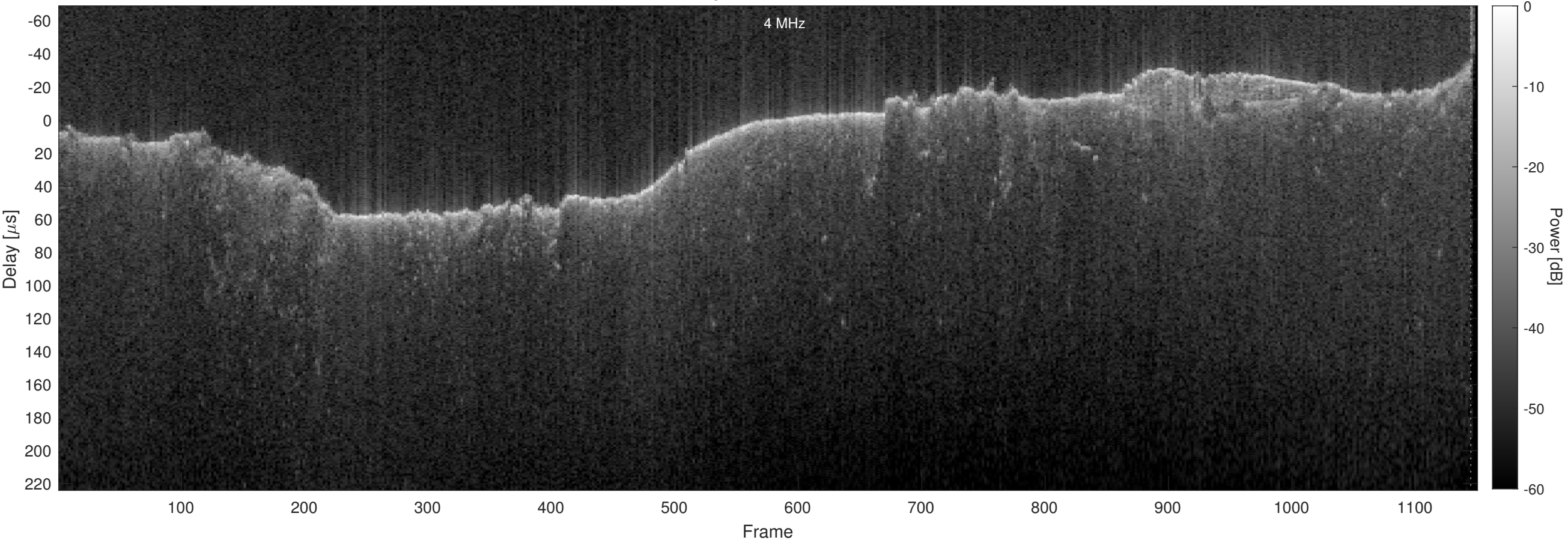
Orbit 15192, Chapman, No Window, Channel 2
