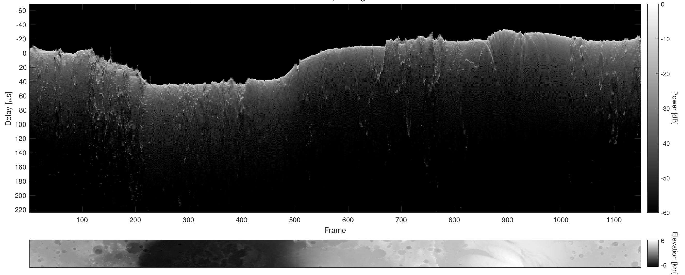
Orbit 15192, Cluttergram
