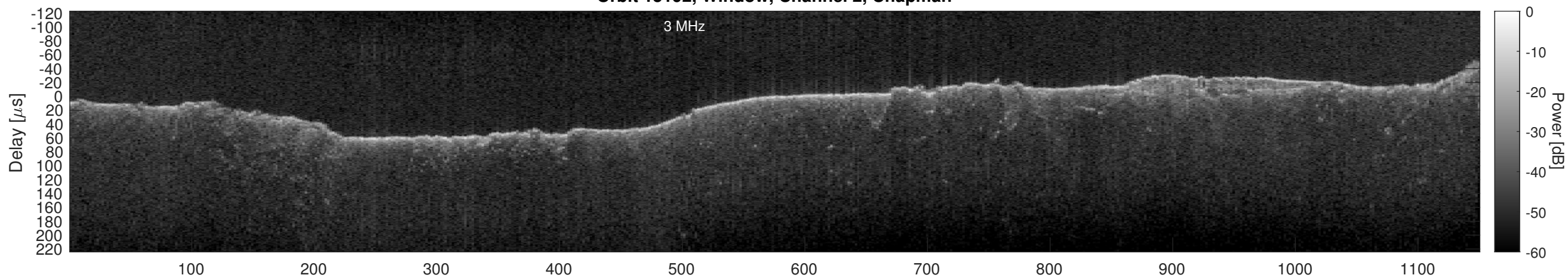
Orbit 15192, Window, Channel 2, Optimized
