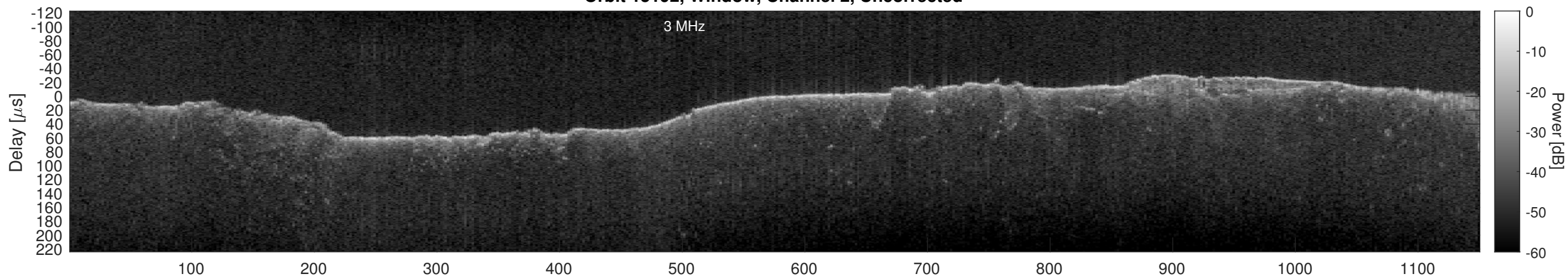
Orbit 15192, Window, Channel 2, Chapman
