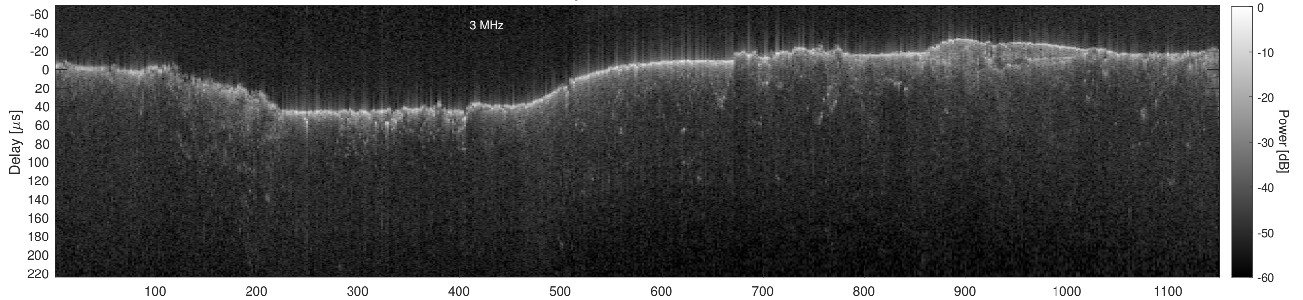
Orbit 15192, Cluttergram
