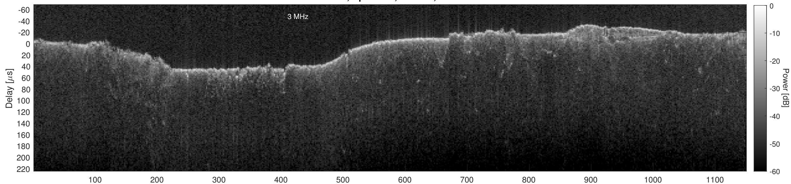
Orbit 15192, Cluttergram
