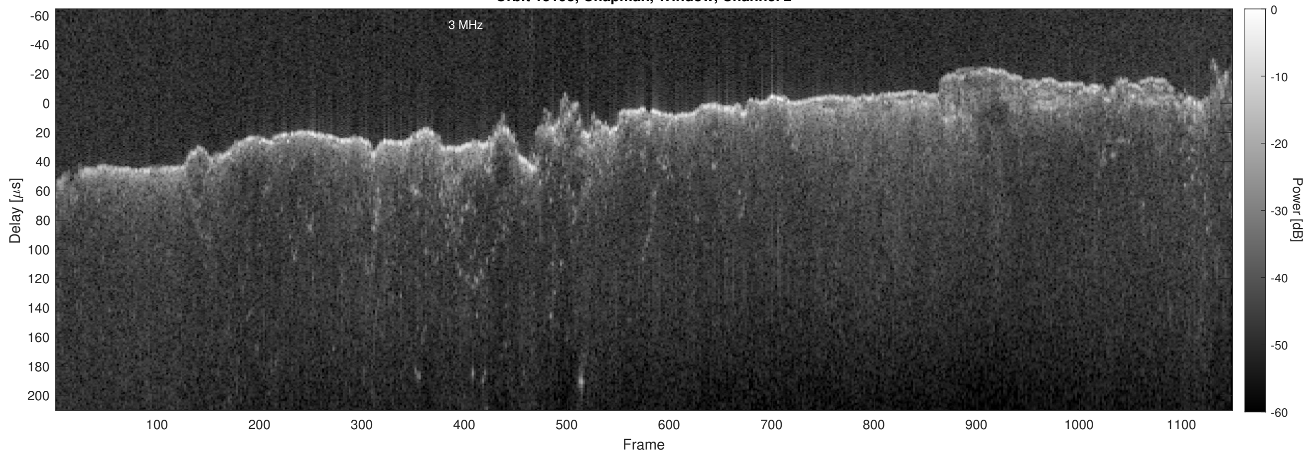
Orbit 15193, Chapman, Window, Channel 2
