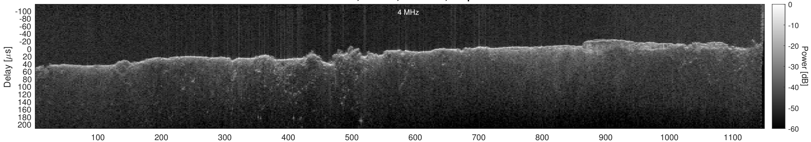
Orbit 15193, Window, Channel 1, Optimized
