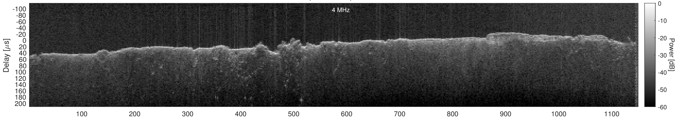
Orbit 15193, Window, Channel 1, Chapman
