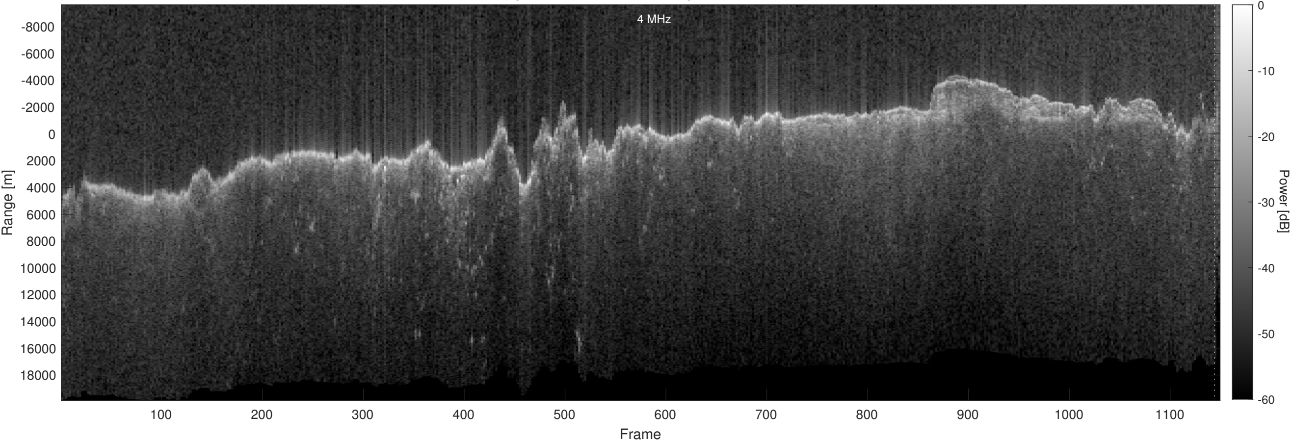
Orbit 15193, Optimized, No Window, Depth-Corrected, Channel 2
