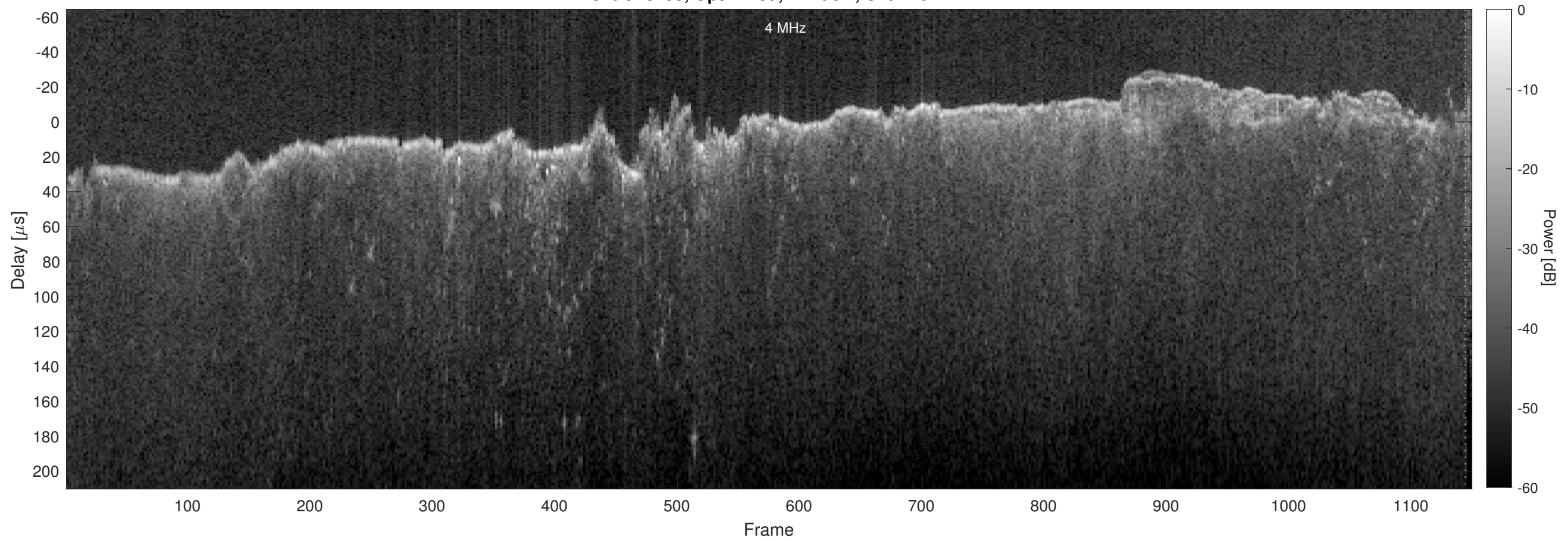
Orbit 15193, Optimized, Window, Channel 2
