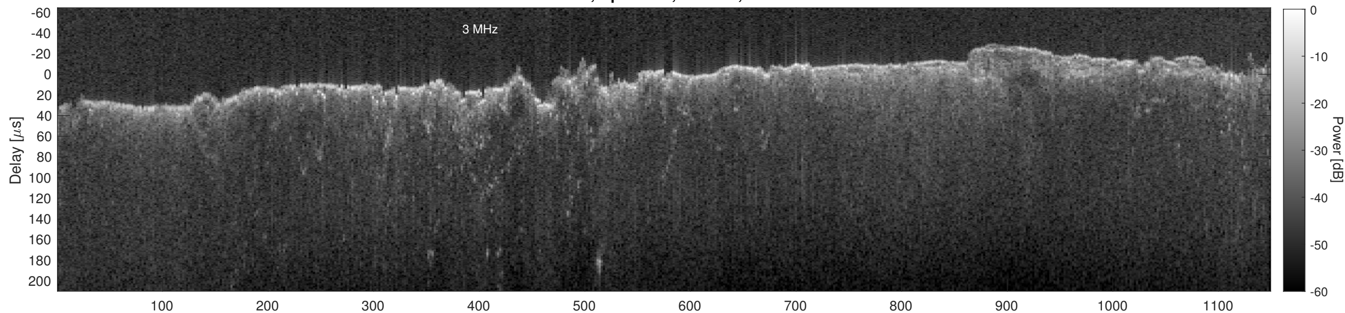
Orbit 15193, Cluttergram
