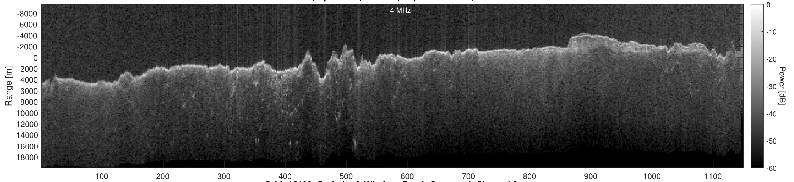
Orbit 15193, Optimized, Window, Depth-Corrected, Channel 2
