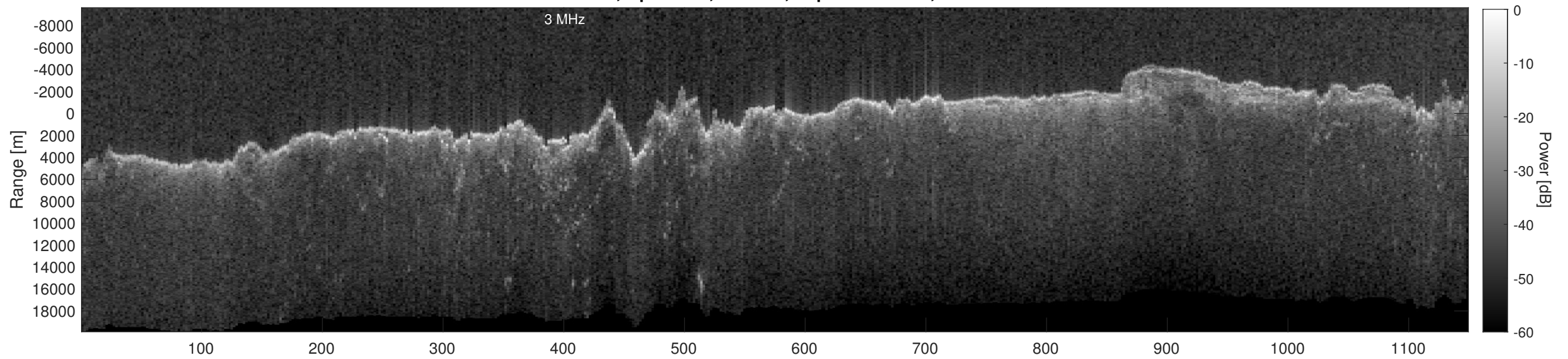
Orbit 15193, Depth-Corrected Cluttergram
