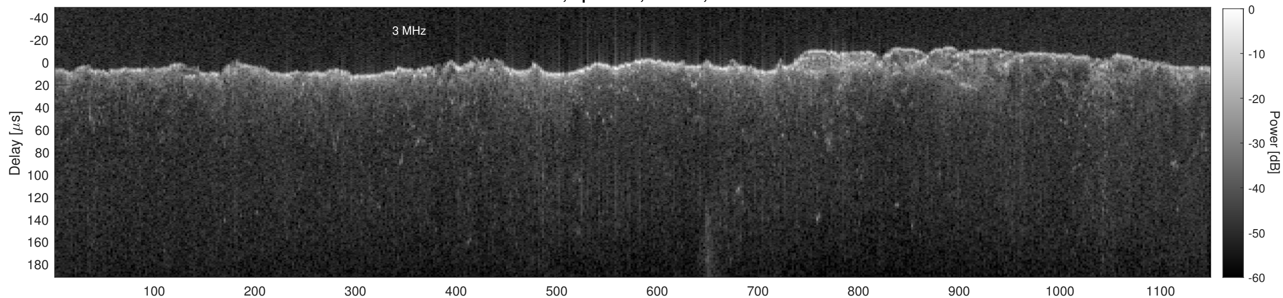
Orbit 15195, Cluttergram
