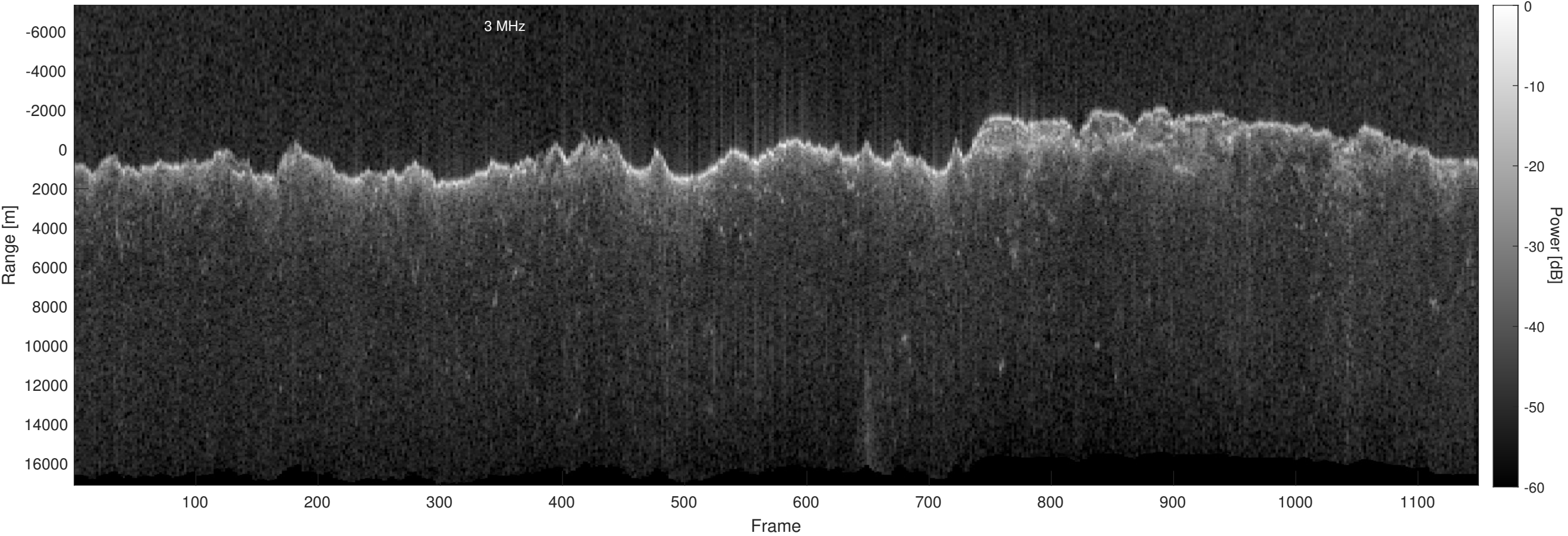
Orbit 15195, Optimized, Window, Depth-Corrected, Channel 2
