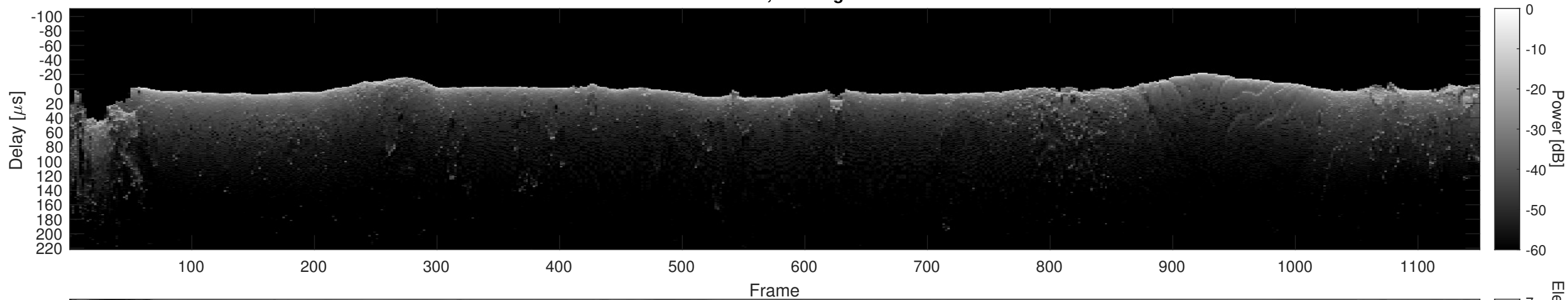
Orbit 15204, Cluttergram
