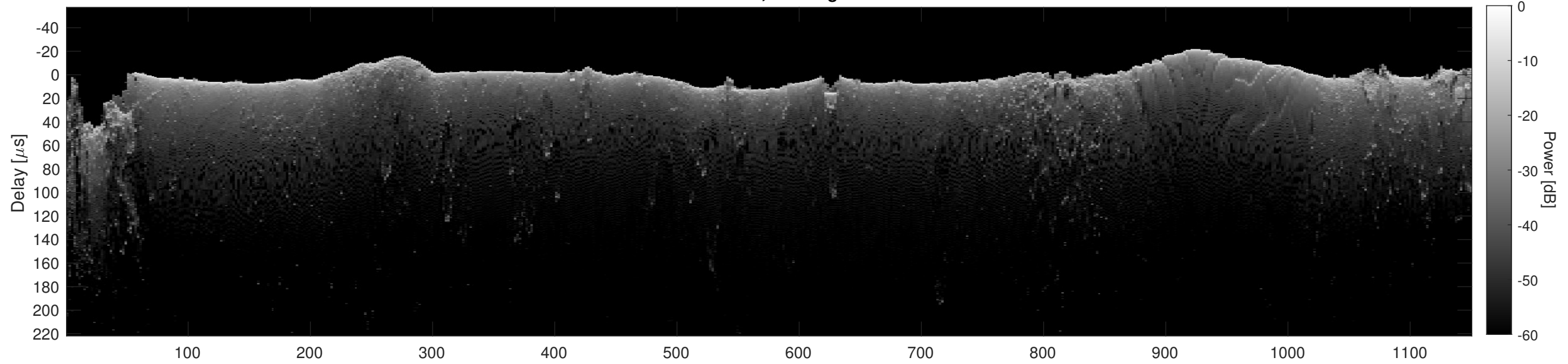
Orbit 15204, Cluttergram
