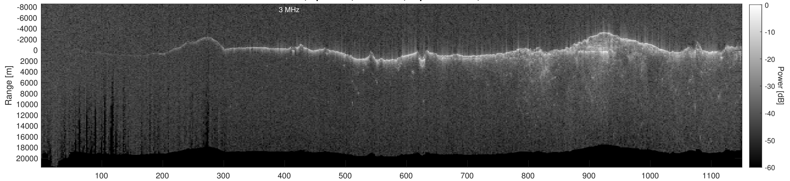
Orbit 15204, Depth-Corrected Cluttergram
