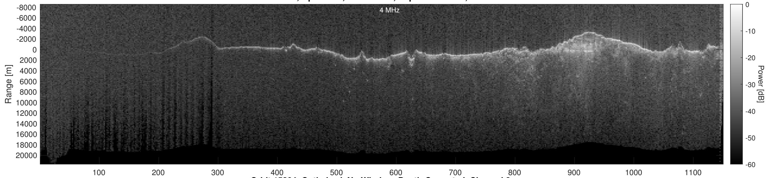
Orbit 15204, Optimized, No Window, Depth-Corrected, Channel 2
