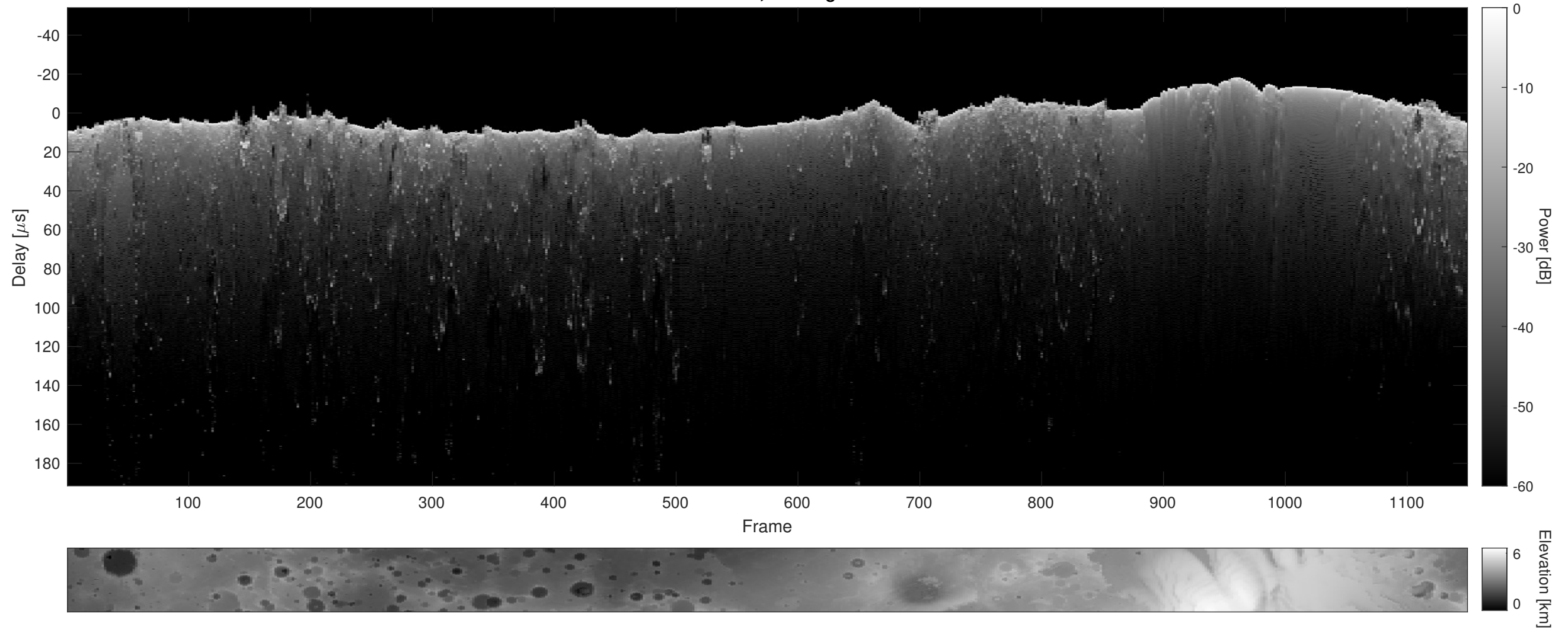
Orbit 15217, Cluttergram
