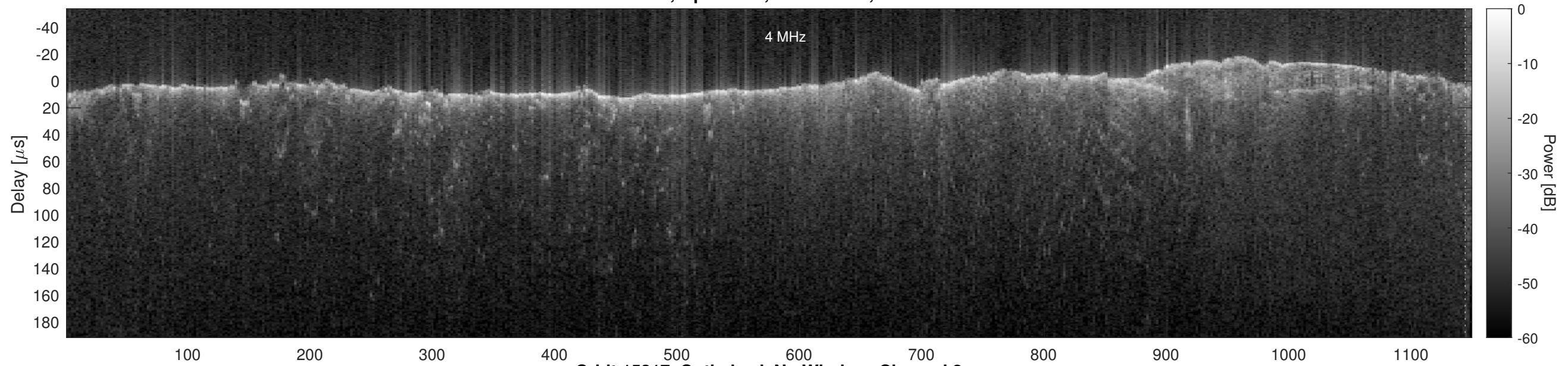
Orbit 15217, Optimized, No Window, Channel 2
