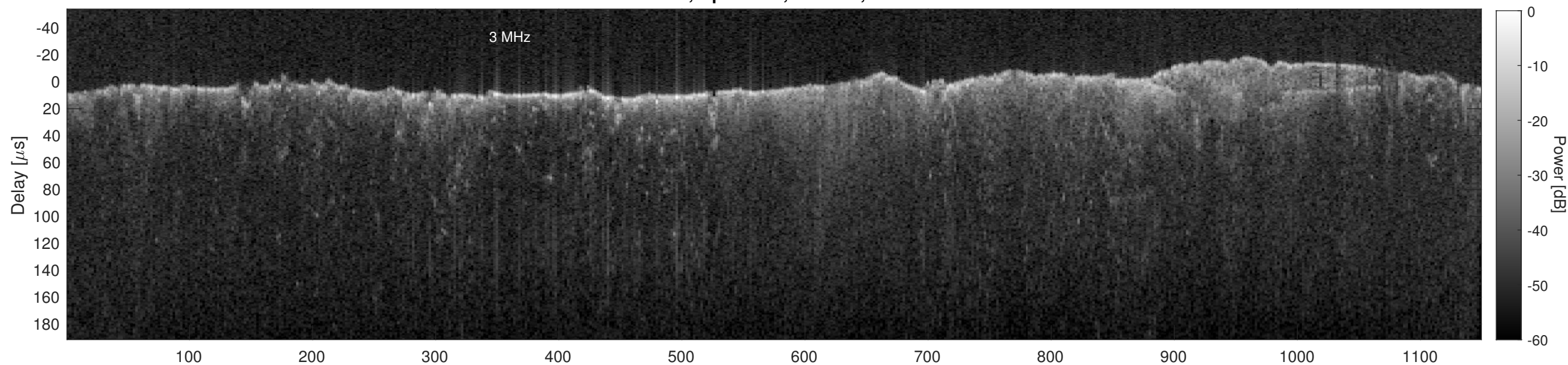
Orbit 15217, Cluttergram
