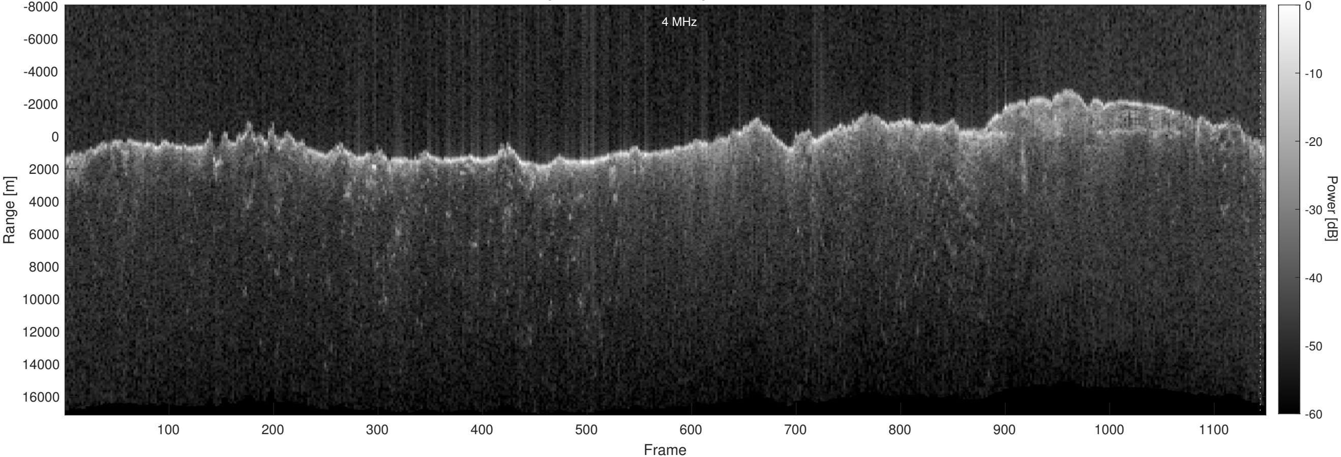
Orbit 15217, Optimized, Window, Depth-Corrected, Channel 2
